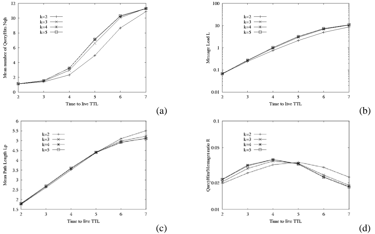
Figure 3. Distribution A. Mean Number of QueryHits (a), Message Load (b), Mean Path Length (c), and QueryHits/Messages ratio (d) w.r.t. the TTL value, for different values of the contact parameter \kappa
