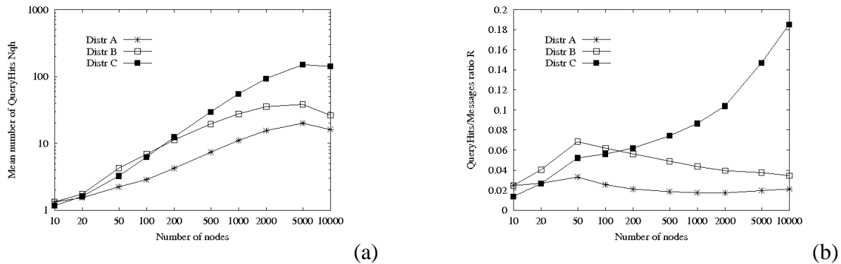
Figure 12. Comparison of Distributions A, B, C. Mean Number of QueryHits (a) and QueryHits/Messages ratio (b) w.r.t. the number of nodes, with TTL=7
