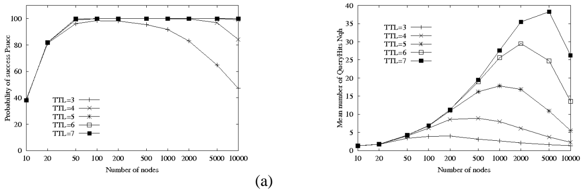
Figure 8. Distribution B. Probability of success (a) and Mean Number of QueryHits (b) w.r.t. the number of nodes, for different values of TTL
