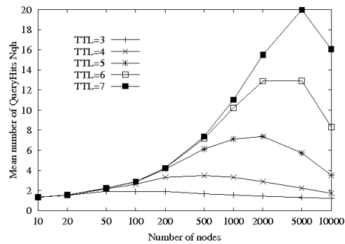
Figure 5. Distribution A. Probability of success (a) and Mean Number of QueryHits (b) w.r.t. the number of nodes, for different values of TTL
