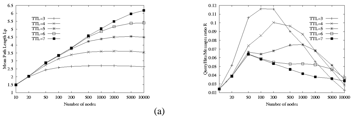
Figure 9. Distribution B. Mean path length (a) and QueryHits/Message ratio (b) w.r.t. the number of nodes, for different values of TTL
