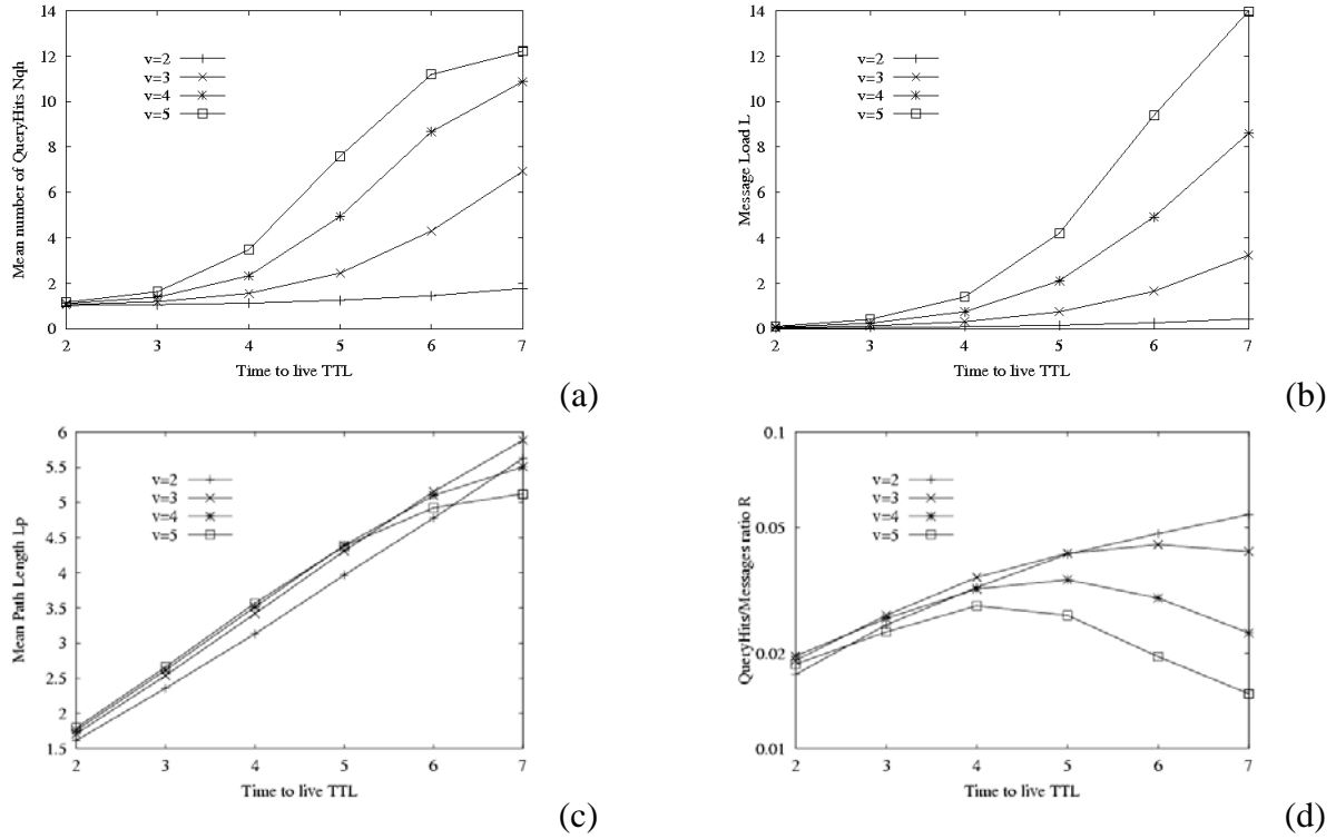
Figure 4. Distribution A. Mean Number of QueryHits (a), Message Load (b) Mean Path Length (c), and QueryHits/Messages ratio (d) w.r.t. the TTL value, for different values of the number of neighbours v .
