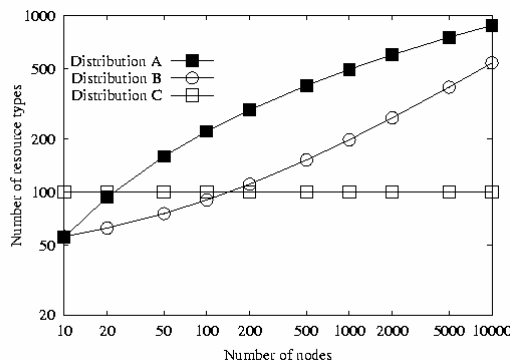
Figure 2. Distributions of resource types used in the protocol analysis.
