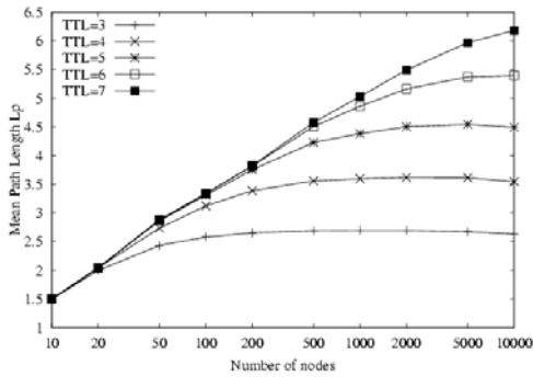
Figure 11. Distribution C. Mean path length (a) and QueryHits/Messages ratio (b) w.r.t. the number of nodes, for different values of TTL
