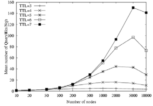
Figure 10. Distribution C. Probability of success (a) and Mean Number of QueryHits (b) w.r.t. the number of nodes, for different values of TTL
