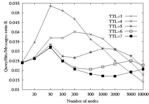
Figure 6. Distribution A. Mean path length (a) and QueryHits/Messages ratio (b) w.r.t. the number of nodes, for different values of TTL
