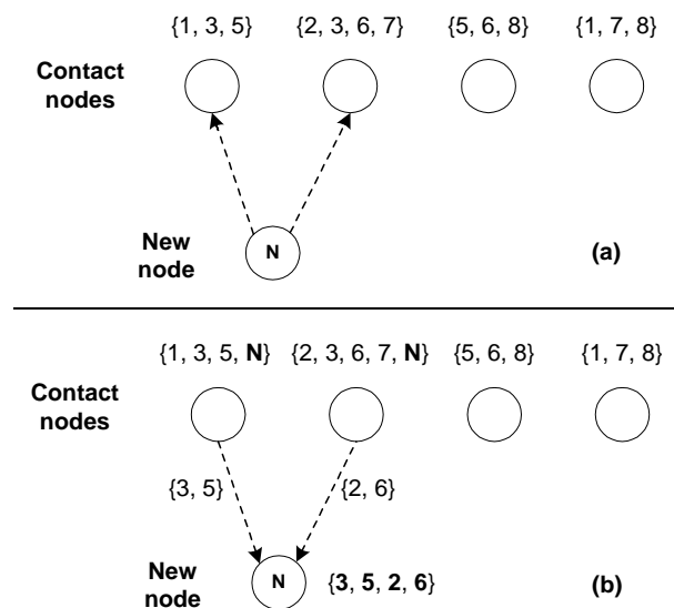
Figure 1. The membership management protocol: a new node joins the P2P network.
